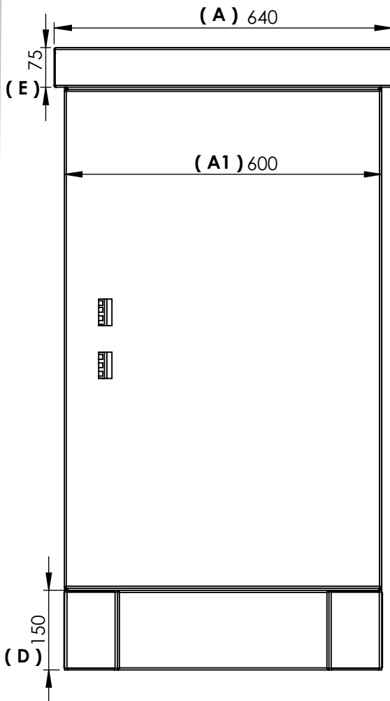
Vista Frontal
